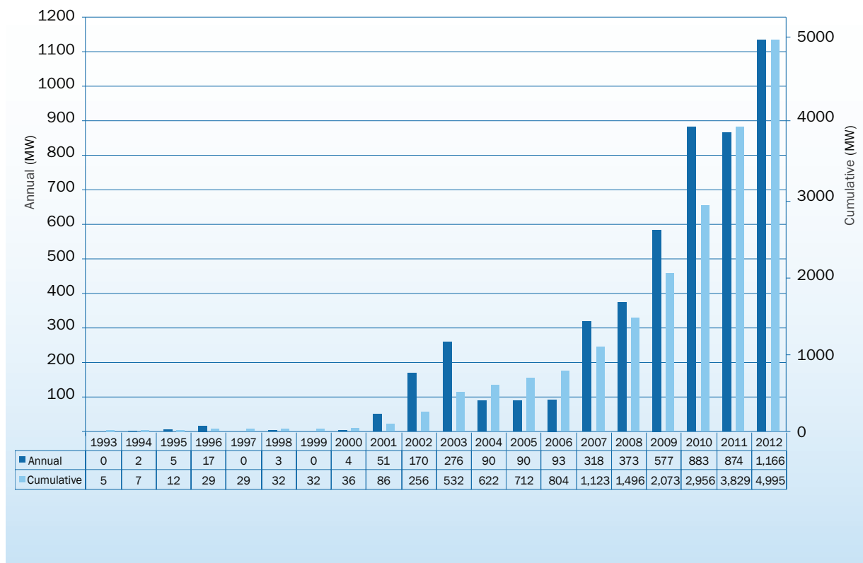
FIG 11: CUMULATIVE AND ANNUAL OFFSHORE WIND INSTALLATIONS (MW).
