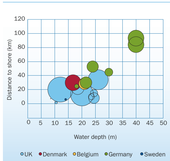
FIG 10: WATER DEPTH, DISTANCE TO SHORE AND SIZE OF OFFSHORE WIND FARMS UNDER CONSTRUCTION DURING 2012
