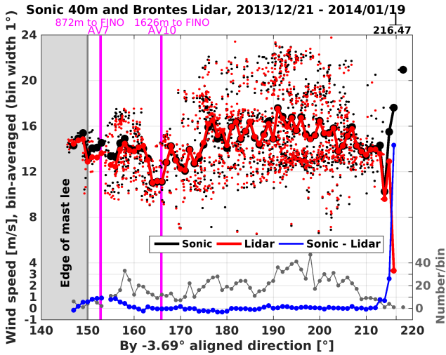
Fig. 7: Red and black dots, small: 10-min mean values, big; direction-bin averaged. Blue dots: Sonic-to-Lidar differences. Lidar-to-Sonic differences for 3 different direction sectors are given in the text.
