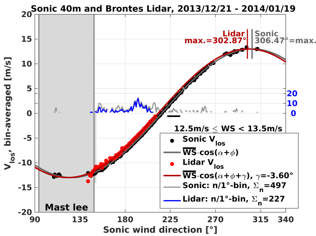
Fig. 5: The shift between the sinusoidal curves for the Sonic and the Lidar in the wind speed bin 12.5-13.5m/s is \gamma = -3.60^\circ . The amplitude of the sinusoidal is equal to the bin centre ( 13m/s ).
