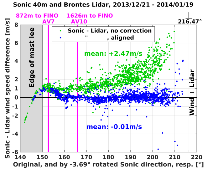
Fig. 8: Sonic to Lidar wind speed differences before (green dots), and after alignment (blue dots).
