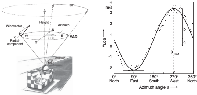
Fig. 1: Left: sketch of the VAD-Lidar scan technique. Right: the measured line-of-sight speeds are arranged on a sinusoidal curve. [2]
