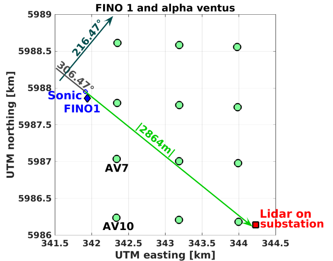
Fig. 4: Measurement setting in wind farm alpha ventus, consisting of 12 5MW-turbines. We'll see, that turbine AV7 has influenced the measurements, but AV10 did not.
