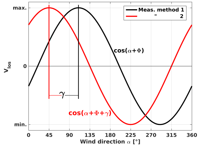
Fig. 2: The V_{los} of two measurement devices, orientated to different direction, are shifted by the angle \gamma . The angle \Phi is explained in the text.
