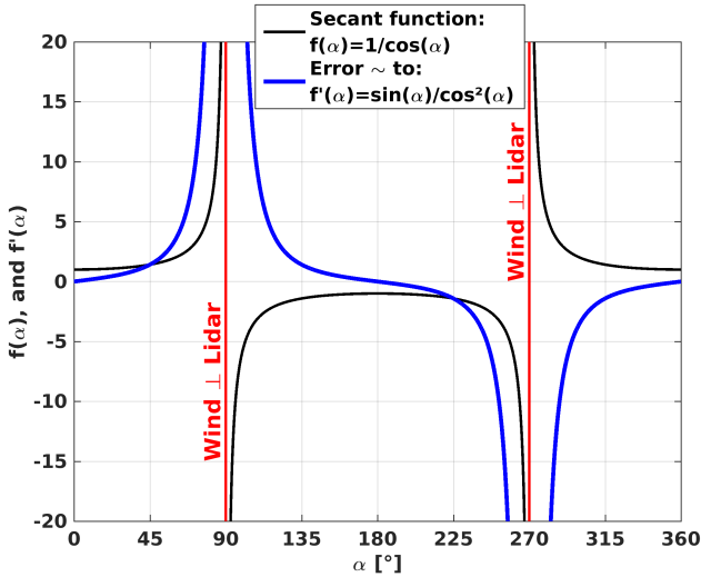
Fig. 3: Closer to angles \alpha=90^\circ and 270^\circ (wind direction is perpendicular to Lidar beam), the derivative of the secant function is growing faster than the secant function itself.
