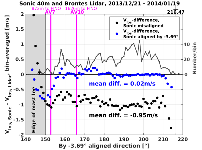
Fig. 6: The aligning procedure reduces the V_{los} -difference considerably. The Sonic data suffer from the mast shadow more than the Lidar data do.
