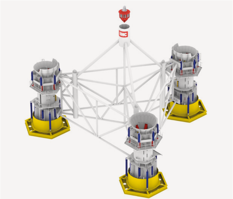
TEMPLATE INCLINATION STICK-UP FOR PILE POSITIONING AND PRE-PILING FOR JACKETS
